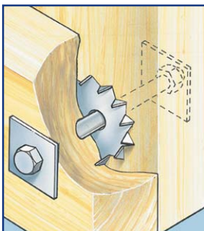
TOOTH PLATE SINGLE SIDED
