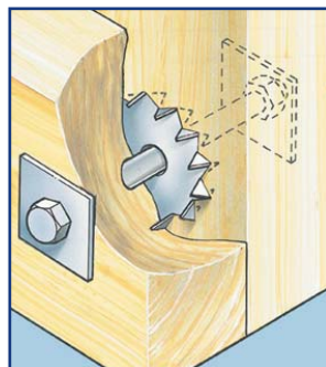
TOOTH PLATE DOUBLE SIDED
